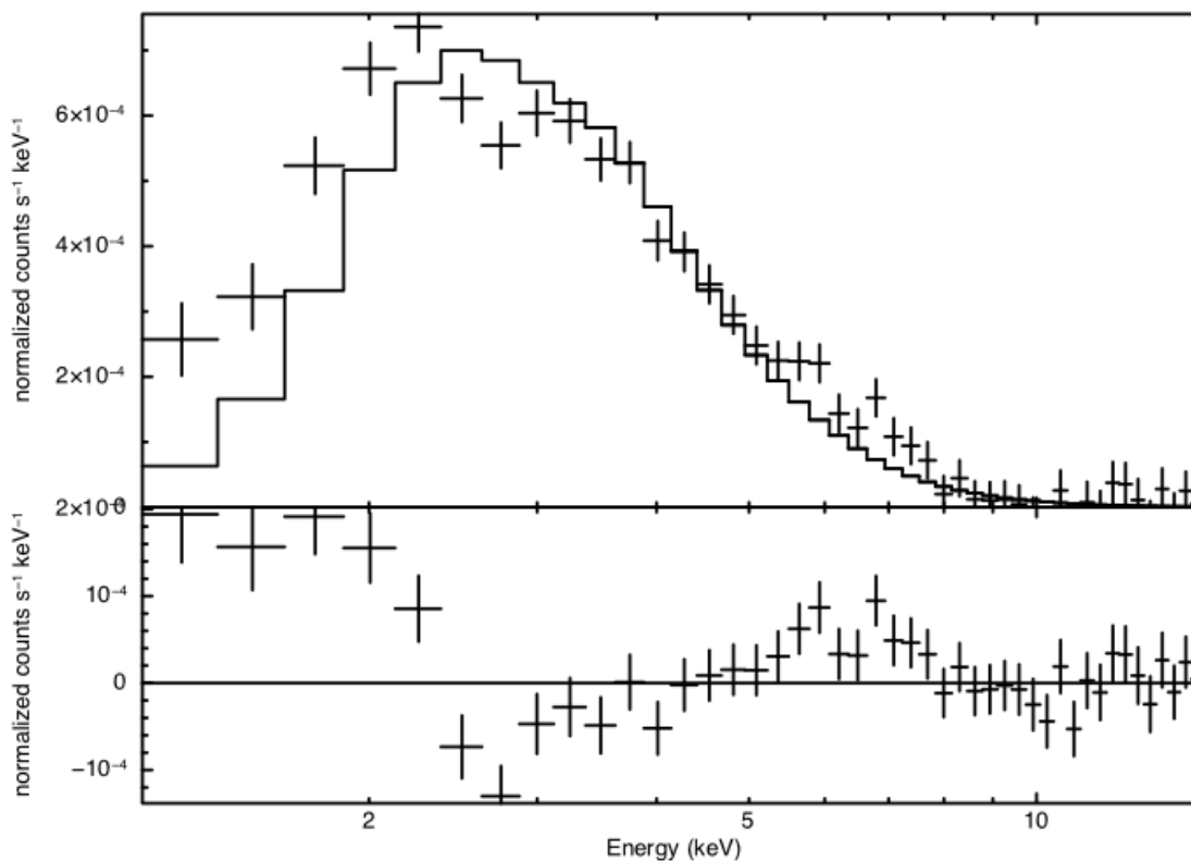
Figure G: As for Figure D & F, but the model is the best-fitting power law with the absorption fixed at the Galactic value. Under the assumptions that the absorption really is the same as the 21-cm value and that the continuum really is a power law, this plot provides some indication of what other components might be added to the model to improve the fit.
