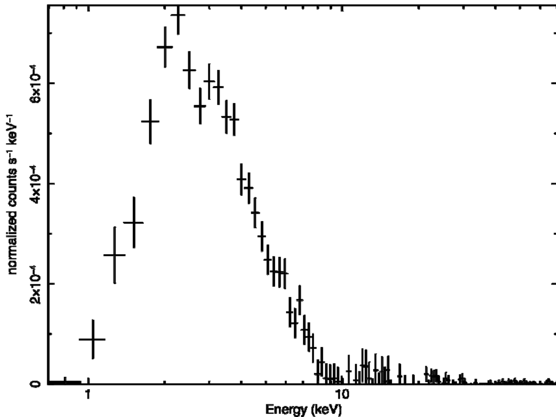
Figure A: The result of the command plot data when the data file in question is the EXOSAT ME spectrum of the 6s X-ray pulsar 1E1048.1--5937 available from the HEASARC on-line service
