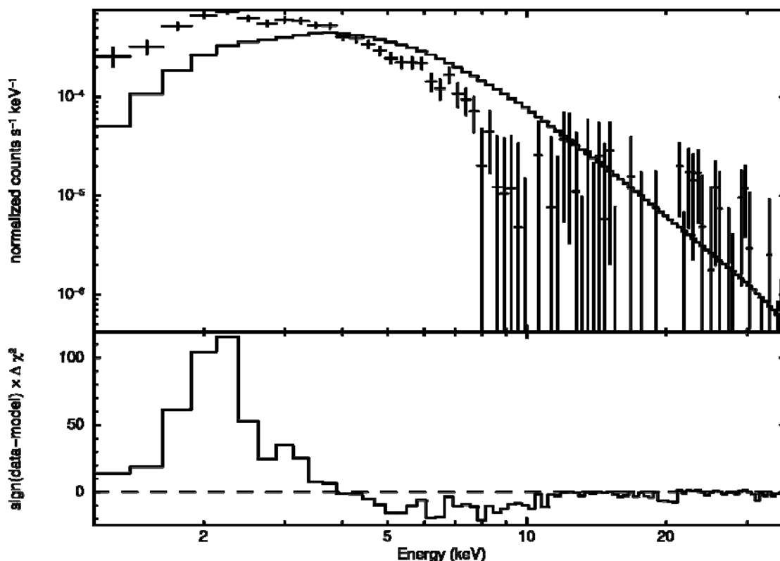
Figure B: The result of the command plotdata chi after the command ignore bad on the EXOSAT ME spectrum 1E1048.1–5937
