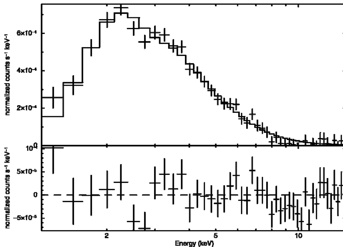
Figure D: The result of the command plot data resid with: the ME data file from 1E1048.1—5937; “bad” and negative channels ignored; the best-fitting absorbed power-law model; the residuals of the fit.
