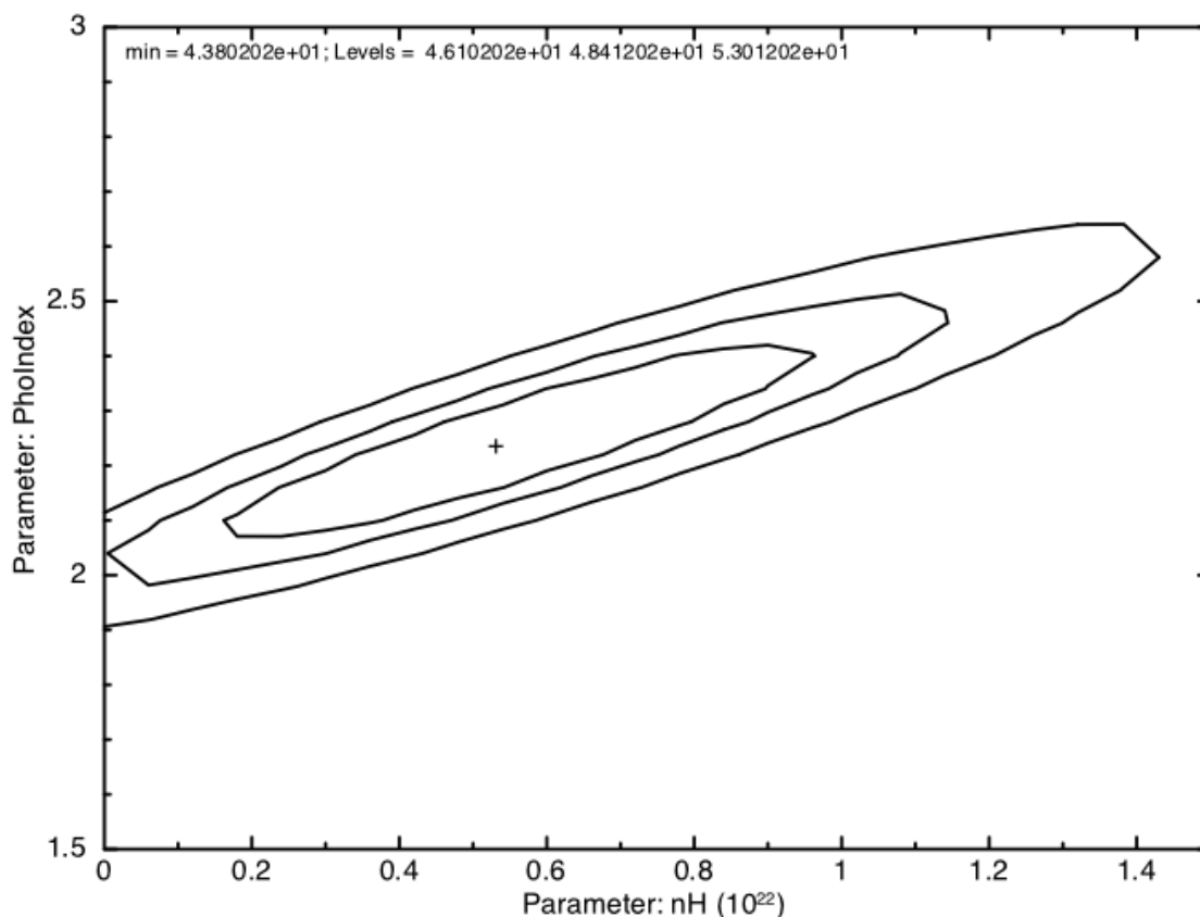
Figure E: The result of the command plot contour. The contours shown are for one, two and three sigma. The cross marks the best-fit position.
