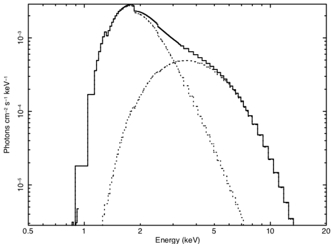
Figure H: The result of the command plot model in the case of the ME data file from 1E1048.1—5937. Here, the model is the best-fitting combination of power law, black body and fixed Galactic absorption. The three lines show the two continuum components (absorbed to the same degree) and their sum.
