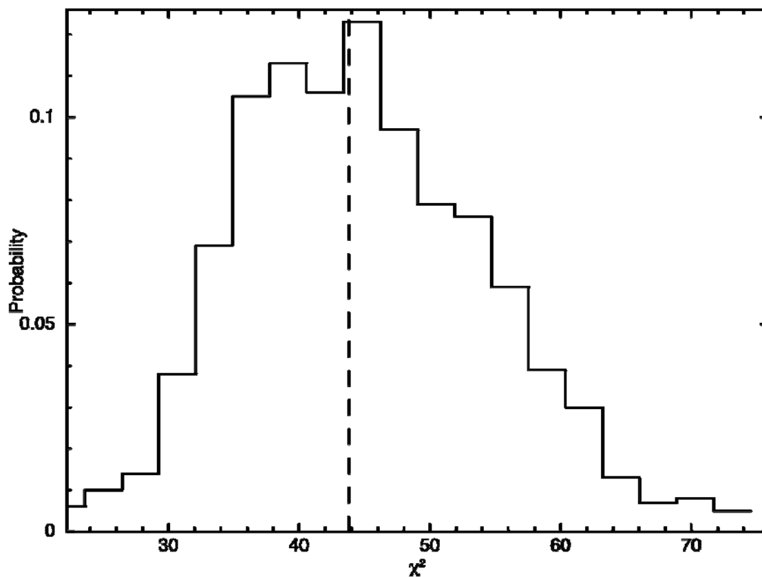
Figure C: The result of the command plot goodness. The histogram shows the fraction of simulations with a given value of the statistic and the dotted line marks that for the observed data. There is no reason to reject the model.
