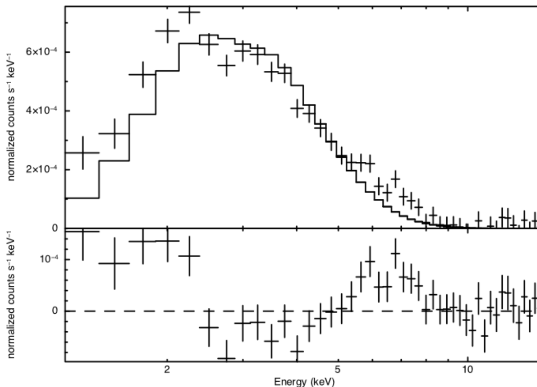
Figure F: As for Figure D, but the model is the best-fitting absorbed black body. Note the wave-like shape of the residuals which indicates how poor the fit is, i.e. that the continuum is obviously not a black body.
