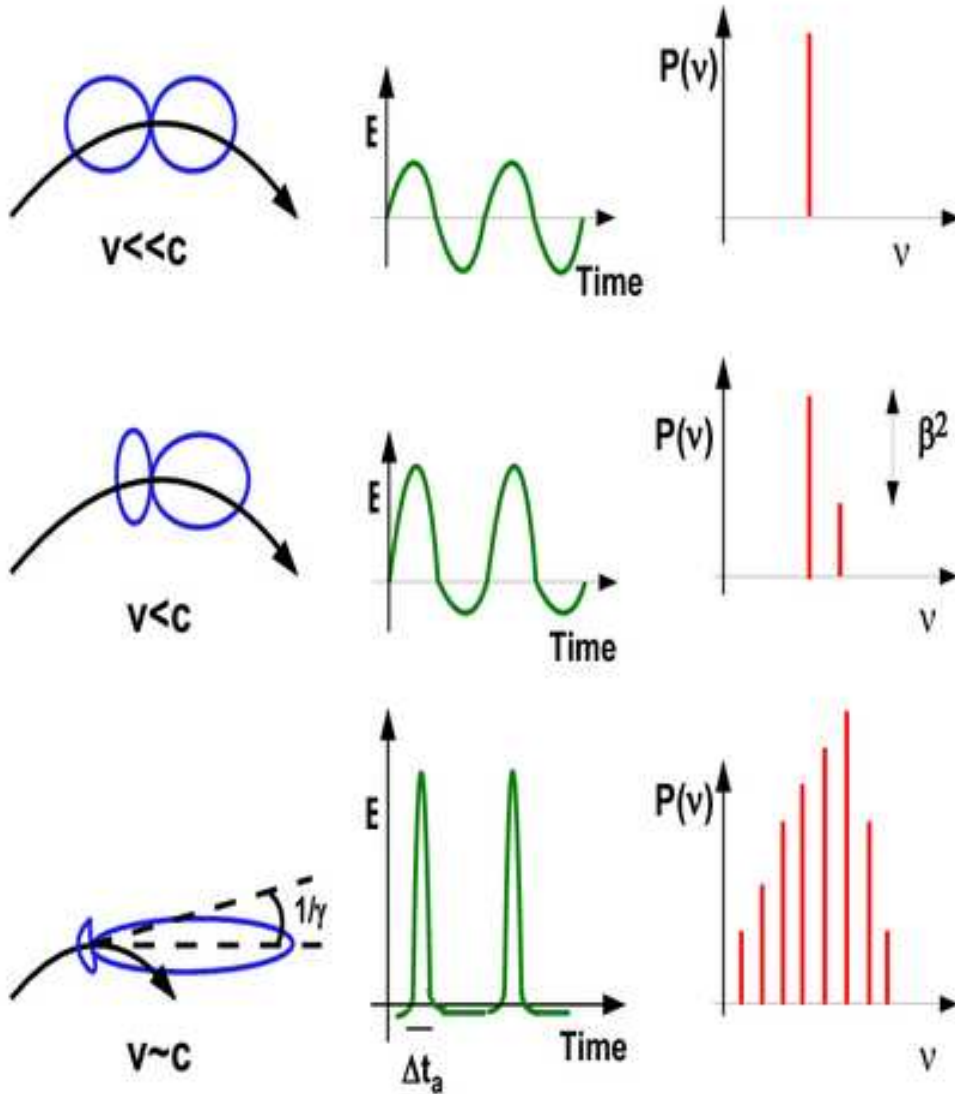
Figure 2.5: From cyclo to synchro: if the emitting particle has a very small velocity, the observer sees a sinusoidal (in time) electric field E(t) . Increasing the velocity the pattern becomes asymmetric, and the second harmonic appears. For 0 < \beta \ll 1 the power in the second harmonic is a factor \beta^2 less than the power in the first. For relativistic particles, the pattern becomes strongly beamed, the emission is concentrated in the time \Delta t_A . As a consequence the Fourier transformation of E(t) must contain many harmonics, and the power is concentrated in the harmonics of frequencies \nu \sim 1/\Delta t_A . Broadening of the harmonics due to several effects ensures that the spectrum in this case becomes continuous. Note that the fundamental harmonic becomes smaller increasing \gamma (since \nu_B \propto 1/\gamma ).
