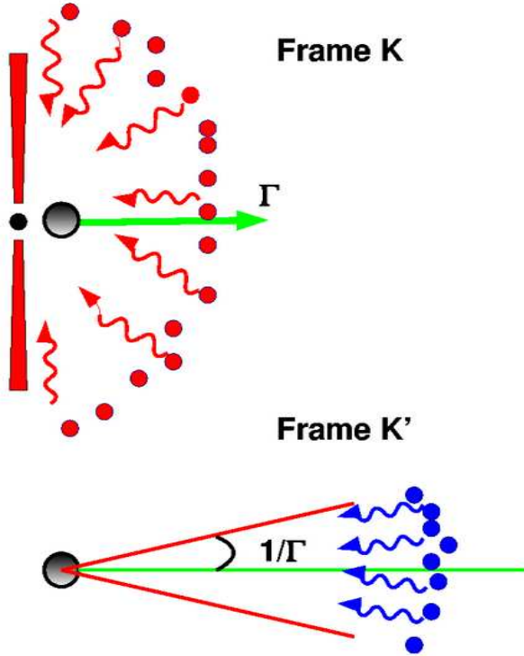
Figure 1.8: A real case: a relativistic bob is moving with the Broad Line Region of a radio loud AGN, with Lorentz factor \Gamma . In the rest frame K' of the blob the photons coming from 90^\circ in frame K are seen to come at an angle 1/\Gamma . The energy density as seen by the blob is enhanced by a factor \sim \Gamma^2 .
