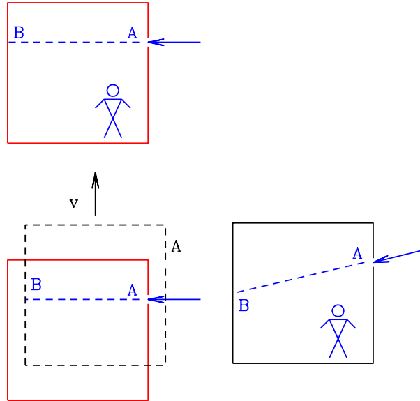
Figure 1.5: The relativistic lift, to explain relativistic aberration of light. Assume first a non-moving lift, with a hole on the right wall. A light ray, coming perpendicularly to the left wall, enters through the wall in A and ends its travel in B . If the lift is moving with a constant velocity v to the top, its position is changed when the photon arrives to the left wall. For the comoving observer, therefore, it appears that the light path is tilted, since the point B where the photon smashes into the left wall is below the point A . What happens if the lift, instead to move with a constant velocity, is accelerating?
