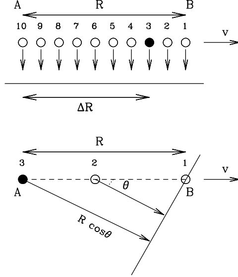
Figure 1.7: Due to the differences in light travel time, the number of blobs that can be observed simultaneously at any given time depends on the viewing angle and the velocity of the blobs. In the top panel the viewing angle is \theta = 90^\circ and all the blobs contained within a certain distance R can be seen. For smaller viewing angles, less blobs are seen. This is because the photons emitted by the rear blobs have more distance to travel, and therefore they have to be emitted before the photons produced by the front blob. Decreasing the viewing angle \theta we see less blobs (3 for the case illustrated in the bottom panel).
