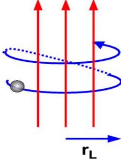
Figure 2.1: A particle gyrates along the magnetic field lines. Its trajectory has an helicoidal shape, with Larmor radius r_L and pitch angle \theta .
