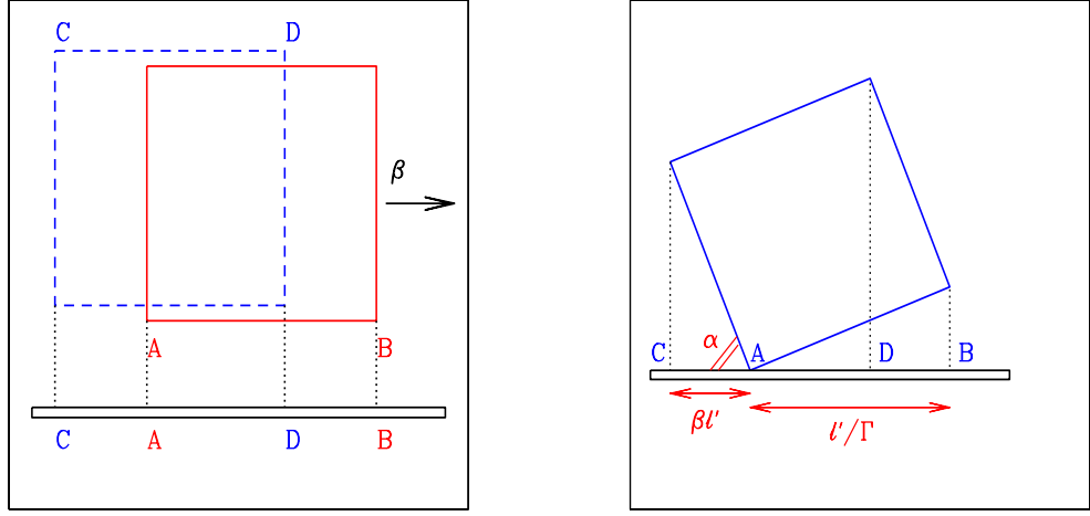
Figure 1.2: Left: A square moving with velocity \beta c seen at 90^\circ . The observer can see the left side (segment CA ). Light rays are assumed to be parallel, i.e. the square is assumed to be at large distance from the observer. Right: The moving square is seen as rotated by an angle \alpha given by \cos \alpha = \beta .
