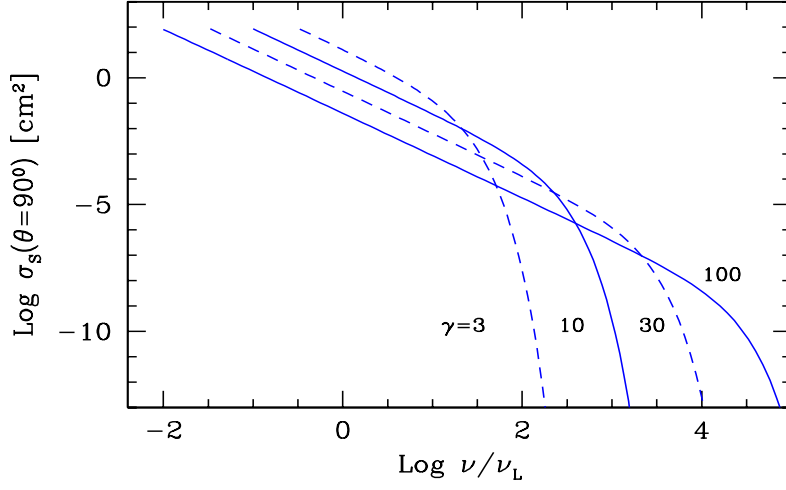
Figure 2.7: The synchrotron absorption cross section as a function of \nu/\nu_L for different values of \gamma , as labeled, assuming a pitch angle of \theta = 90^\circ and a magnetic field of 1 Gauss.
