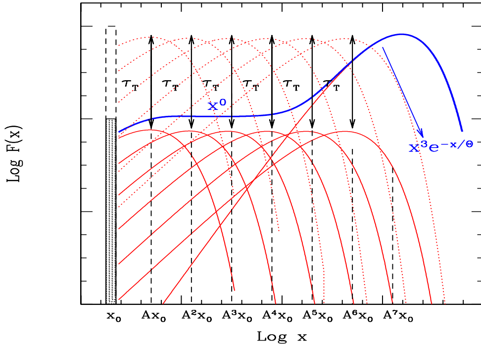
Figure 4.11: Multiple Compton scatterings when \tau_T > 1 and y \gg 1 . For the first scattering orders, nearly all photons are scattered: only a fraction 1/\tau_T can escape. Therefore the number of photons escaping at each scattering order is the same. This is the reason of the flat part, where F(x) \propto x^0 . When the photon frequency is of the order of \Theta , photons and electrons are in equilibrium, and even if only a small fraction of photon can escape at each scattering order, they do not change frequency any longer, and therefore they form the Wien bump , with the slope F(x) \propto x^3 e^{-x/\Theta} . If we increase \tau_T , the flux with slope x^0 decreases, while the Wien bump stays the same.
