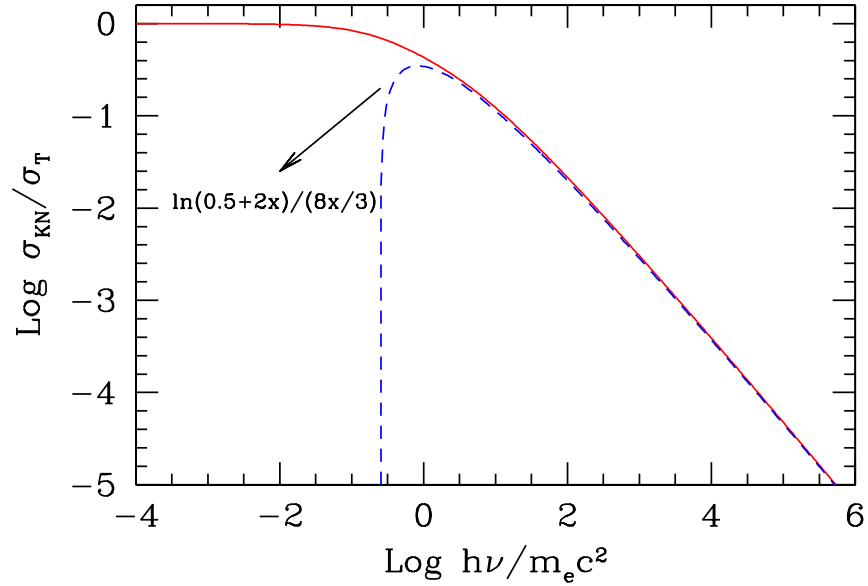
Figure 4.2: The total Klein–Nishina cross section as a function of energy. The dashed line is the approximation at high energies as given in Eq. 4.13.
