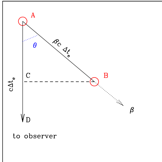
Figure 1.4: Difference between the proper time and the photons arrival time. A lamp, moving with a velocity \beta c , emits photons for a time interval \Delta t'_e in its frame K' . The corresponding time interval measured by an observed at an angle \theta , who receives the photons produced by the lamp is \Delta t_a = \Delta t'_e / \delta .
