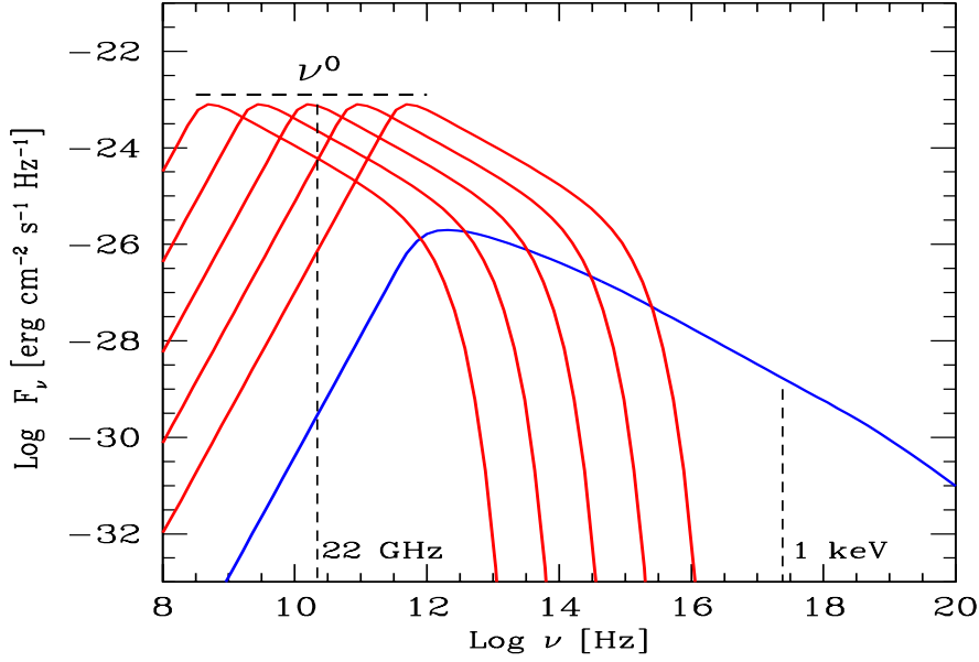
Figure 5.2: Typical example of the composite spectrum of a flat spectrum quasars (FSRQ) shown in the F_\nu vs \nu representation, to better see the flat spectrum in the radio. The reason of the flat spectrum is that different parts of the jet contributes at different frequencies, but in a coherent way. The blue line is the SSC spectrum. Suppose to observe, with the VLBI, at 22 GHz: in this framework we will always observe the jet component peaking at this frequency. So you automatically observe at the self-absorption frequency of that component (for which you measure the angular size).
