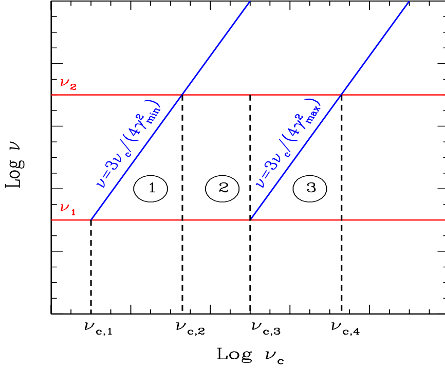
Figure 4.9: The \nu - \nu_c plane. The two diagonal lines delimit the regions of the seed photons that can be used to give a given frequency \nu_c .
