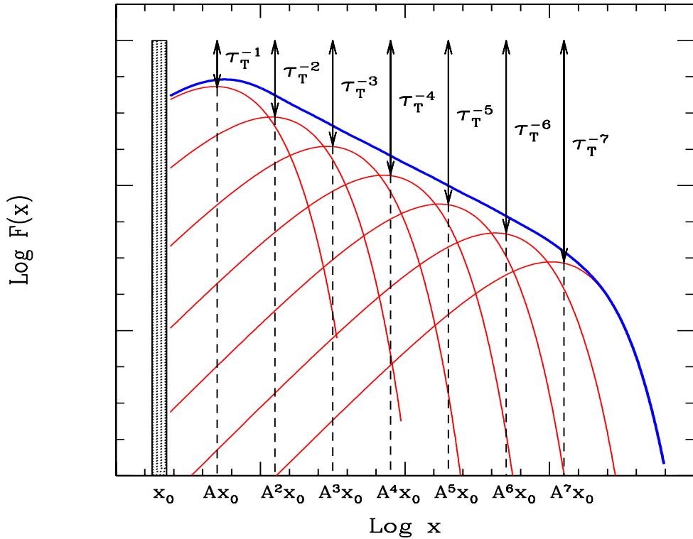
Figure 4.10: Multiple Compton scatterings when \tau_T < 1 . A fraction \tau_T of the photons of the previous scattering order undergoes another scattering, and amplifying the frequency by the gain factor A , until the typical photon frequency equals the electron temperature \Theta . Then further scatterings leave the photon frequency unchanged.
