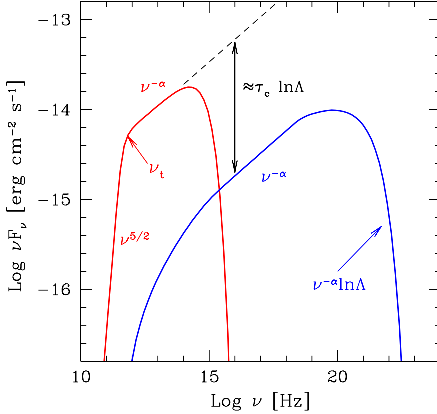
Figure 5.1: Typical example of SSC spectrum, shown in the \nu F_\nu vs \nu representation. The spectral indices instead correspond to the F_\nu \propto \nu^{-\alpha} convention.
