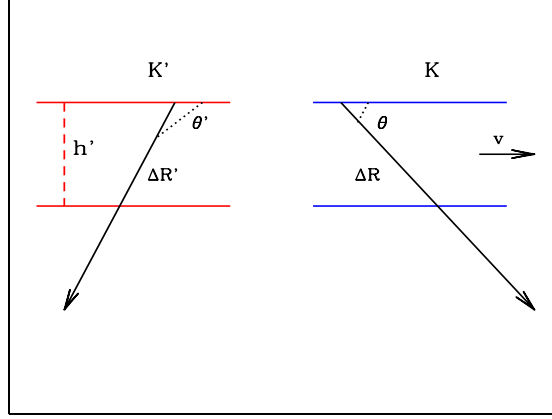
Figure 1.6: Due to aberration of light, the travel path of the a light ray is different in the two frames K and K'
