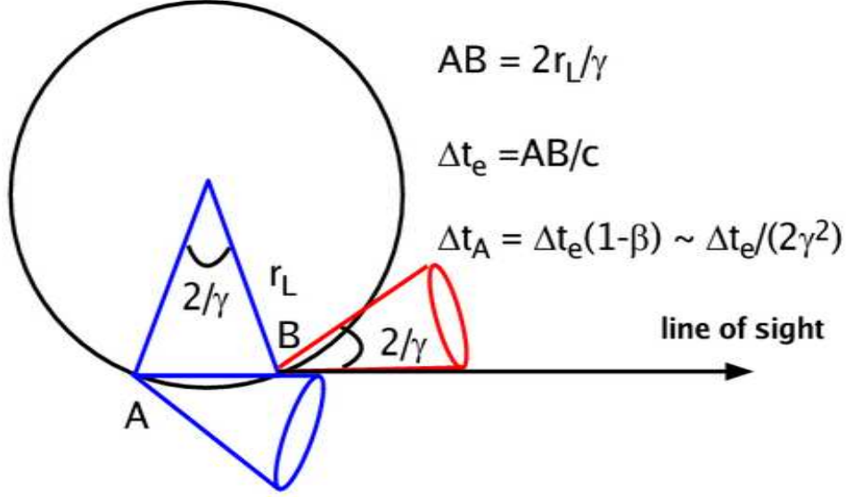
Figure 2.3: A relativistic electron is gyrating along a magnetic field line with pitch angle 90^\circ . Its trajectory is then a circle of radius r_L . Due to aberration, an observer will “see it” (i.e. will measure an electric field) when the beaming cone of total aperture angle 2/\gamma is pointing at him.
