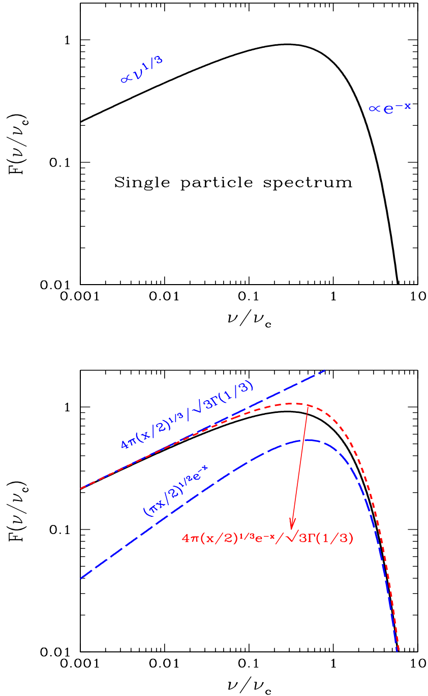
Figure 2.4: Top panel: The function F(\nu/\nu_c) describing the synchrotron spectrum emitted by the single electron. Bottom panel: F(\nu/\nu_c) is compared with some approximating formulae, as labeled. We have defined x \equiv \nu/\nu_c .
