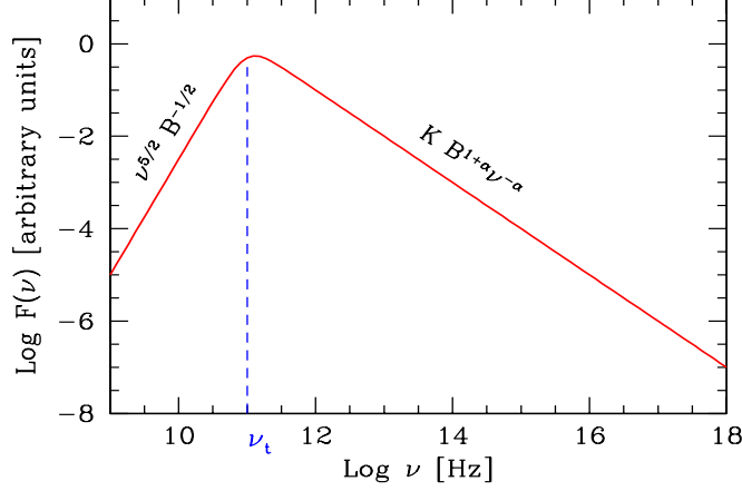
Figure 2.6: The synchrotron spectrum from a partially self absorbed source. Observations of the self absorbed part could determine B . Observations of the thin part can then determine K and the electron slope p .
