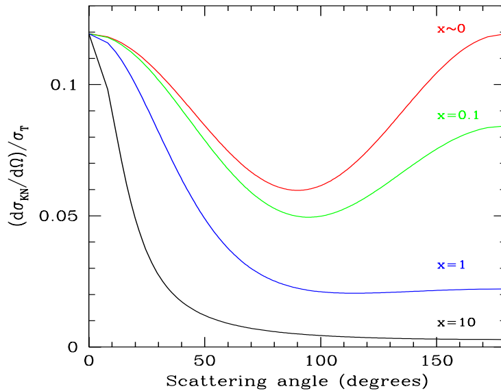
Figure 4.3: The differential Klein–Nishina cross section (in units of \sigma_T ), for different incoming photon energies. Note how the scattering becomes preferentially forward as the energy of the photon increases.
