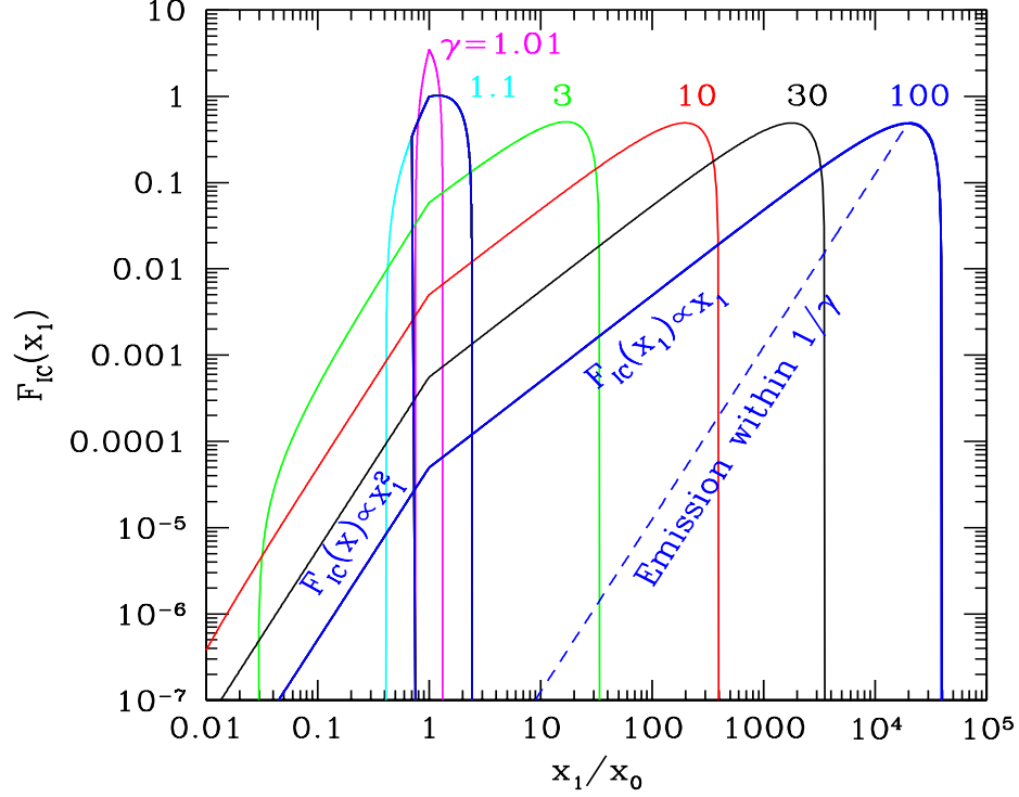
Figure 4.8: Spectrum emitted by the Inverse Compton process by electrons of different \gamma (as labeled) scattering an isotropic monochromatic radiation field of dimensionless frequency x_0 . The dashed line corresponds to the spectrum emitted within the 1/\gamma beaming cone: it always contains the 75% of the total power, for any \gamma . For x_1 < x_0 we have downscattering , i.e. the photons lose energy in the process. Note also the power law segments arising when \gamma \gg 1 : F_{\text{IC}}(x_1) \propto x_1^2 for the downscattering tail, and F_{\text{IC}}(x_1) \propto x_1 for the upscattering segment.
