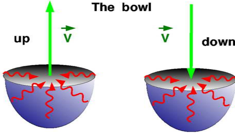
Figure 4.7: In the center of a semi-sphere (the “bowl”) we have relativistic electrons going down and going up, all with the same \gamma . Since the seed photon distribution is anisotropic, so is the scattered radiation and power. The losses of the electron going down are 7 times larger than those of the electron going up (if \gamma \gg 1 ). Since almost all the radiation is produced along the velocity vector of the electrons, also the downward radiation is 7 times more powerful than the upward radiation.
