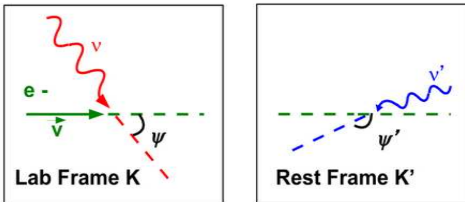
Figure 4.5: In the lab frame an electron is moving with velocity \mathbf{v} . Its velocity makes an angle \psi with an incoming photon of frequency \nu . In the frame where the electron is at rest, the photon is coming from the front, with frequency \nu' , making an angle \psi' with the direction of the velocity.
