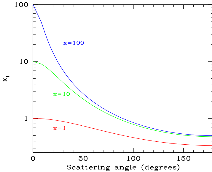
Figure 4.4: Scattered photon energies as a function of the scattering angle, for different incoming photon energies. Note that, for x \gg 1 and for large scattering angle, the scattered photon energies becomes x_1 \sim 1/2 , independent of the initial photon energy x .
