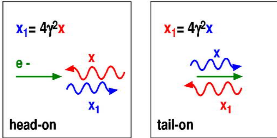
Figure 4.6: Minimum and maximum scattered frequencies. The maximum occurs for head-on collisions, the minimum for tail-on ones. These two frequencies are one the inverse of the other.
